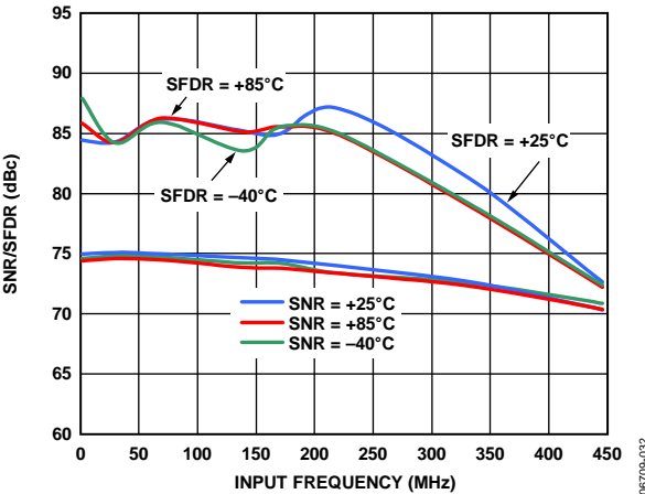
Figure 33. AD6655-125 Single-Tone SNR/SFDR vs. Input Frequency ( f_{IN} ) and Temperature with DRVDD = 1.8 \text{ V}
